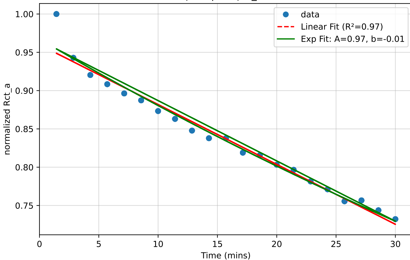
Chip 53 | 100pM_disso
