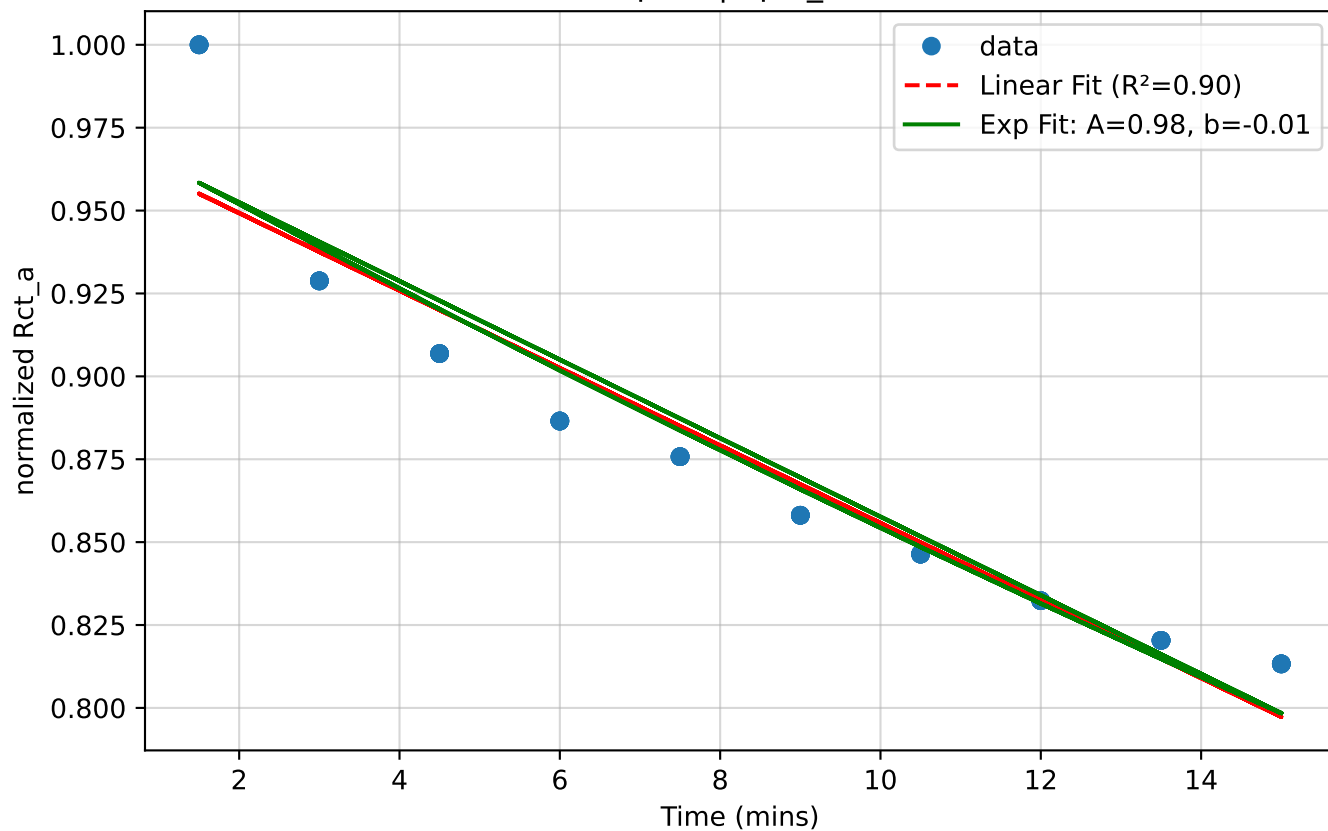
Chip 46 | 0pM_asso
