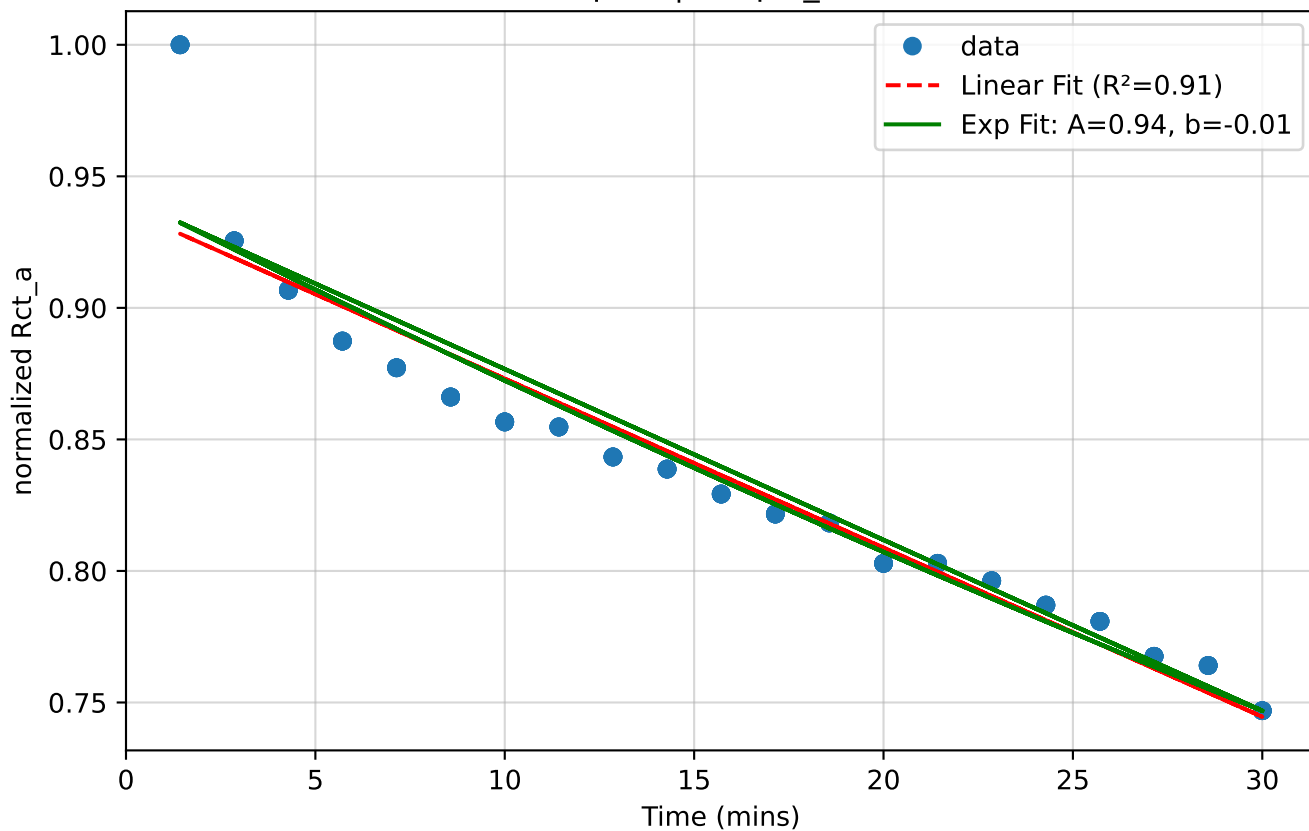
Chip 46 | 100pM_disso
